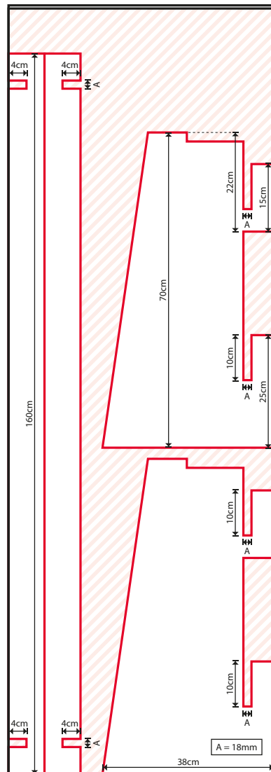
OSB-PANEL 2
