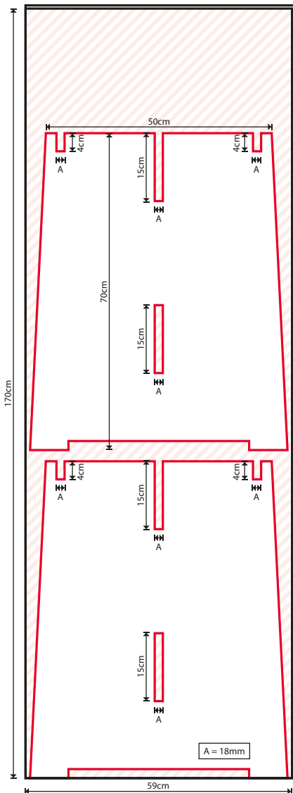
OSB-PANEL 1
